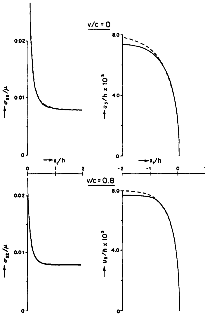
Fig. 2. Comparison of numerical (—) and analytical (---) solutions of \sigma_{32} and u_3 in the plane of the crack in a perfectly elastic strip for v/c = 0 and v/c = 0.8
